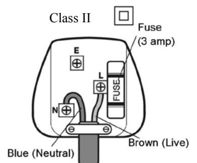
Plug wiring diagram
